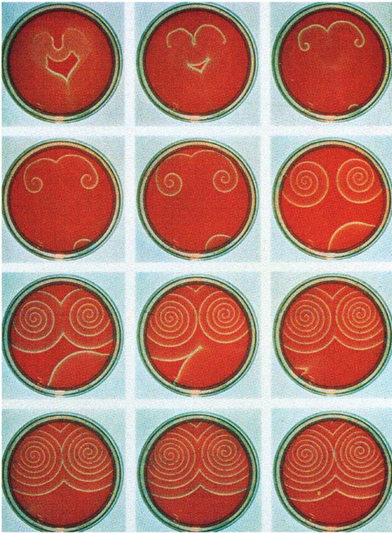
Plate 1: Spiral waves of chemical activity in a shallow dish of the Belousov- Zhabotinsky reaction ( Section 8.3 ). These snapshots read from left to right and top to bottom. The complicated initial condition shown in the upper left was
