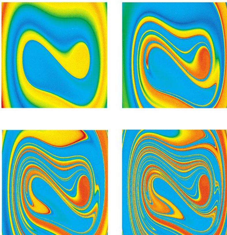
Plate 4: Maps of the short-term behavior of the periodically forced double-well oscillator. Equations, parameters, and color code as in Plate 3 . However, instead of showing the system's asymptotic behavior, these plates show the color-coded value of x(t) after only 1, 2, 3, and 4 drive cycles, respectively. The red and blue regions correspond to initial conditions that converge rapidly to one of the two attractors. A rainbow of colors is found near the basin boundary, because those initial conditions lead to trajectories that linger far from either attractor during the time shown.
