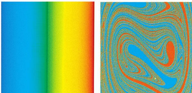
Plate 3: Fractal basin boundaries for the periodically forced double-well oscillator
