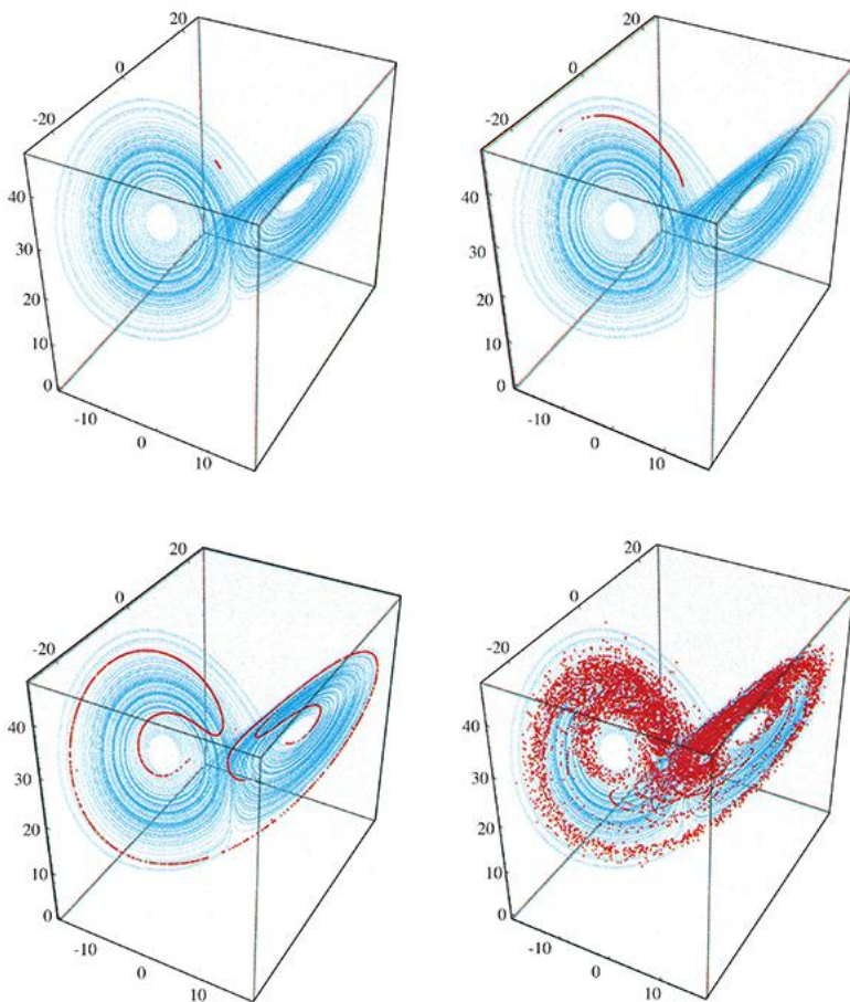
Plate 2: Divergence of nearby trajectories on the Lorenz attractor ( Section 9.3 ). The Lorenz attractor is shown in blue. The red points show the evolution of a small blob of 10,000 nearby initial conditions, at times t = 3, 6, 9 , and 15 . As each point moves according to the Lorenz equations, the blob is stretched into a long thin filament, which then wraps around the attractor. Ultimately the points spread over much of the attractor, showing that the final state could be almost
